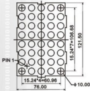
CPM46058
