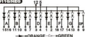
PCB:D18011G/HEG
