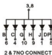
PCB:D5011A/B
