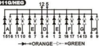
PCB:D18011G/HEG
