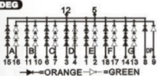
PCB:D18011G/HEG
