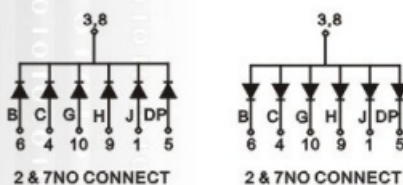
PCB:D5011A/B
